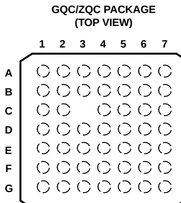
TERMINAL ASSIGNMENTS (1)
