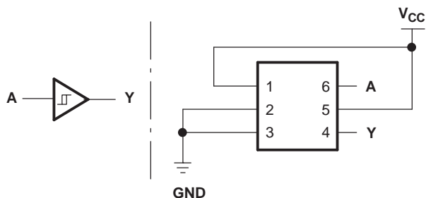
Figure 6. Noninverted Buffer
