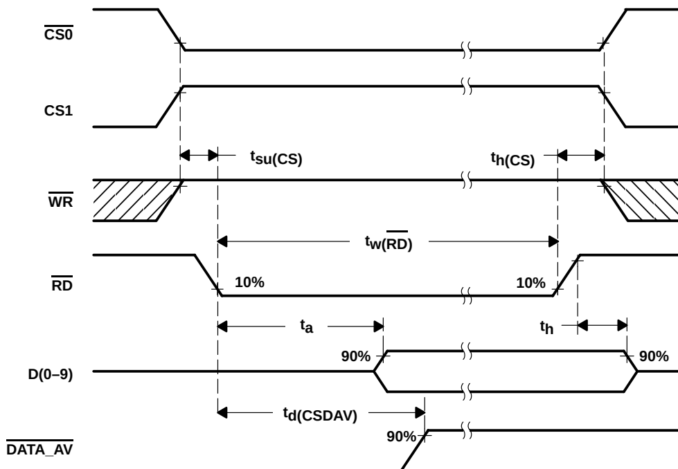
Figure 40. Read Timing Diagram Using \overline{\text{RD}} ( \overline{\text{RD}} -controlled)
