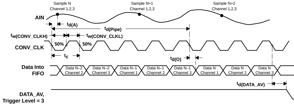
Figure 29. Timing of Continuous Conversion Mode (3-channel operation)
