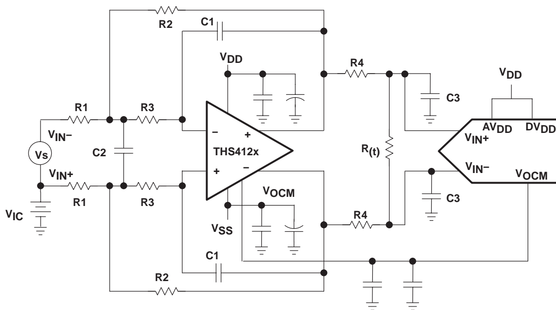
Figure 22. Antialias Filtering
