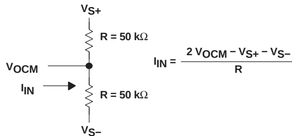
Equivalent Input Circuit for V_{OCM} Figure 101
