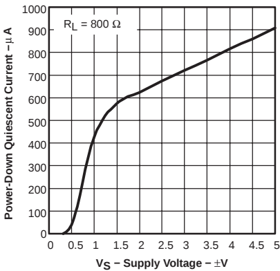
POWER-DOWN QUIESCENT CURRENT VS SUPPLY VOLTAGE
