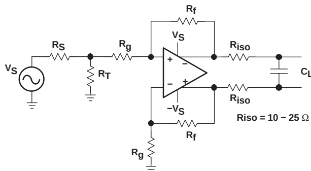
Use of Isolation Resistors With a Capacitive Load. Figure 114
