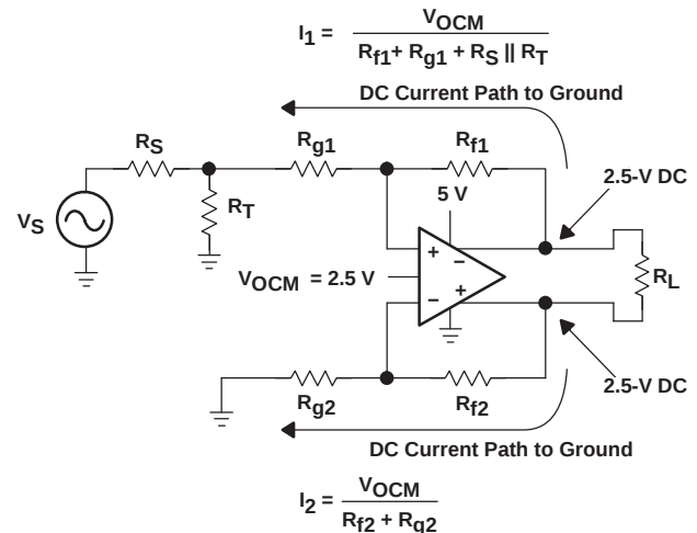
Depiction of DC Power Dissipation Caused By Output Level-Shifting in a DC-Coupled Circuit Figure 102
