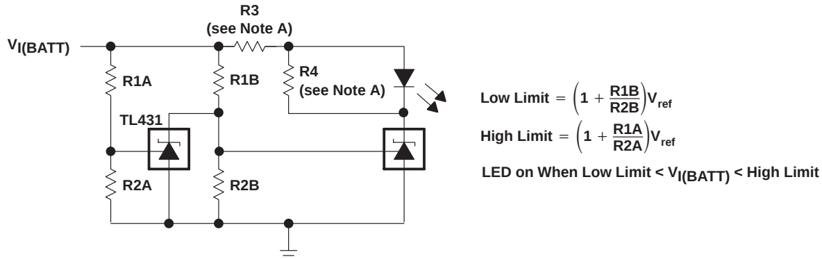
Figure 26. Voltage Monitor
