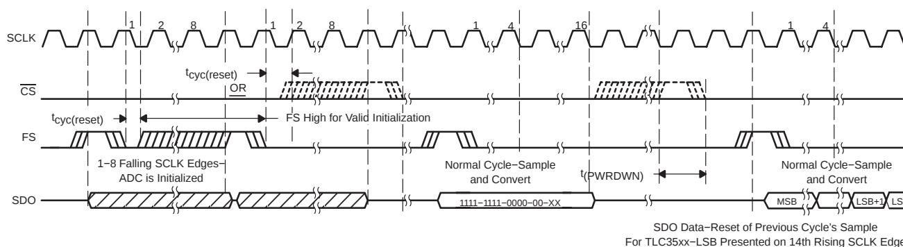
Figure 14. TLC3541/45 Initialization Timing
