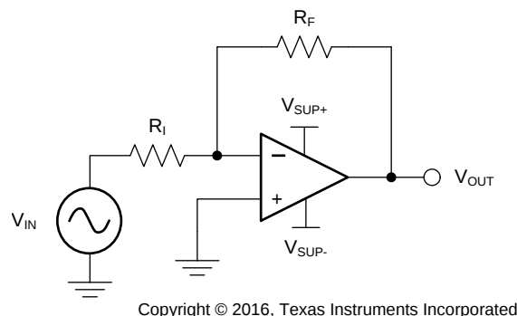
Figure 20. Application Schematic
