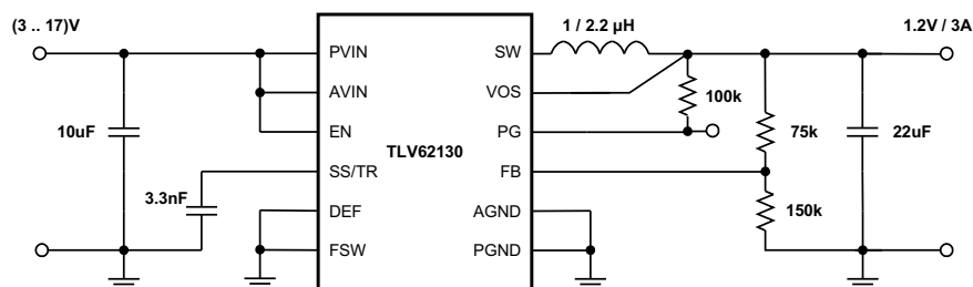
Figure 46. 1.2-V / 3-A Power Supply
