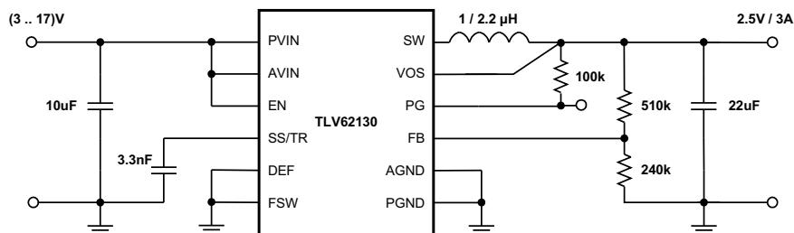
Figure 43. 2.5-V / 3-A Power Supply
