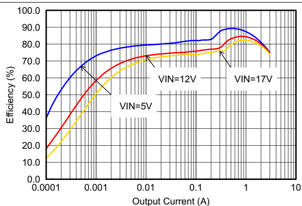
Figure 16. Efficiency With 1.25 MHz, Vout = 1.8 V
