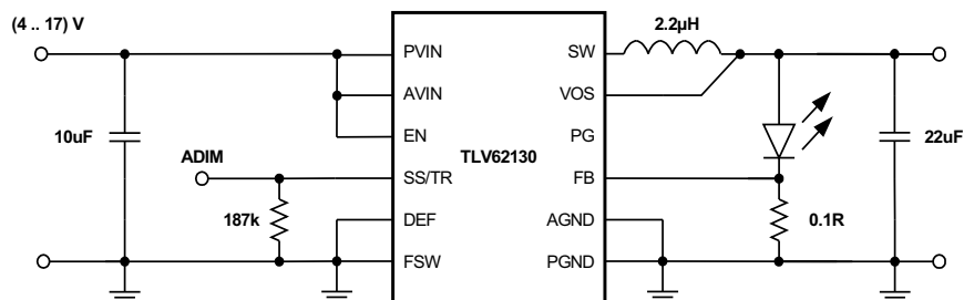
Figure 38. 3 A Single LED Power Supply
