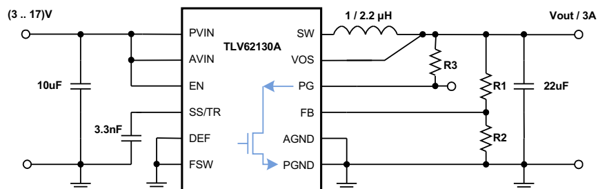
Figure 39. Discharge Vout Through PG Pin With TLV62130A
