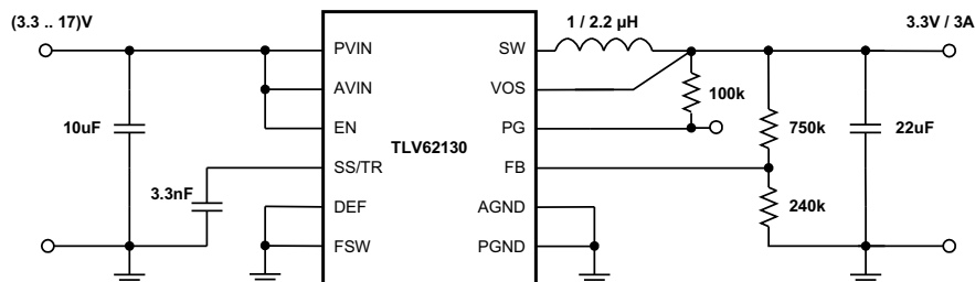
Figure 42. 3.3-V / 3-A Power Supply
