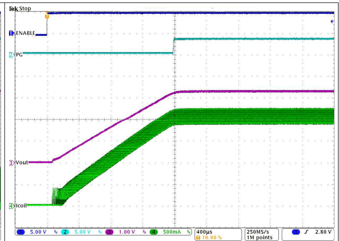
Figure 33. Startup into 3 A
