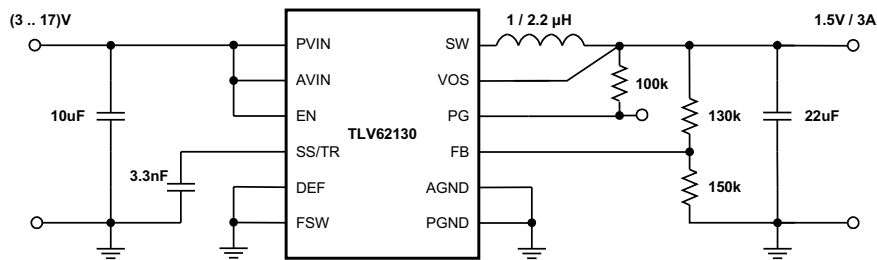
Figure 45. 1.5-V / 3-A Power Supply
