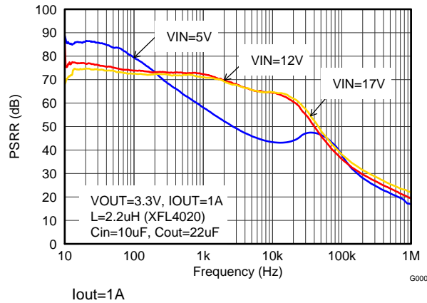
Figure 26. Power Supply Rejection Ratio, F_{SW} = 2.5\text{ MHz}
