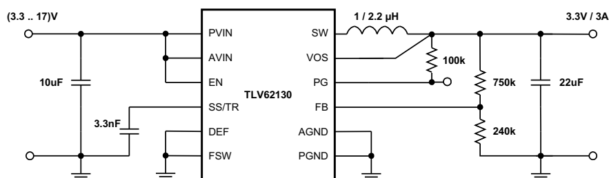
Figure 5. 3.3-V / 3-A Step-Down Converter
