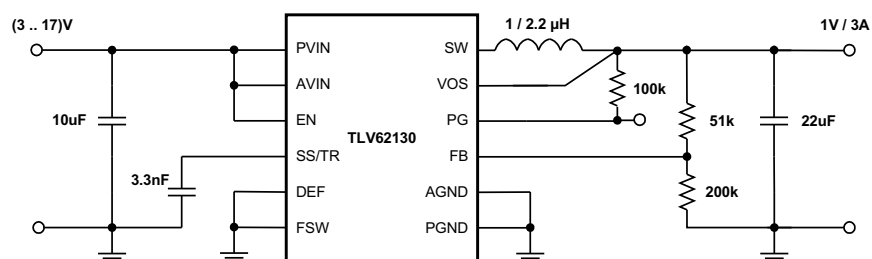
Figure 47. 1-V / 3-A Power Supply
