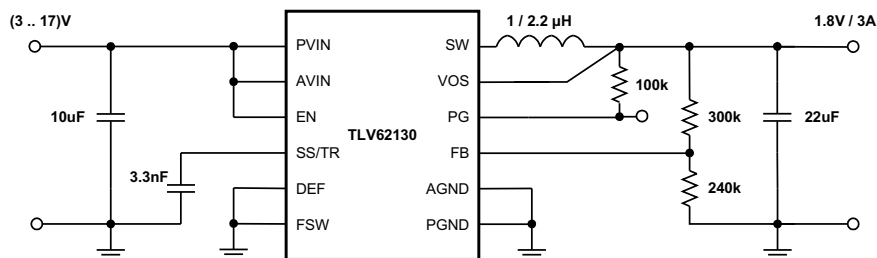
Figure 44. 1.8-V / 3-A Power Supply
