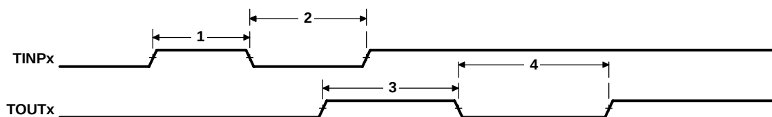
Figure 18–1. Timer Timing
