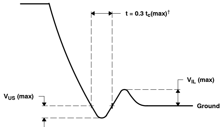
Figure 4–5. AC Transient Specification Fall Time
