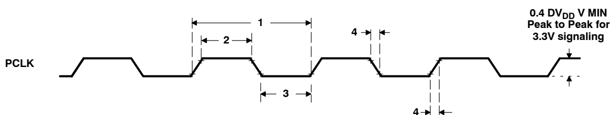
Figure 14–1. PCLK Timing
