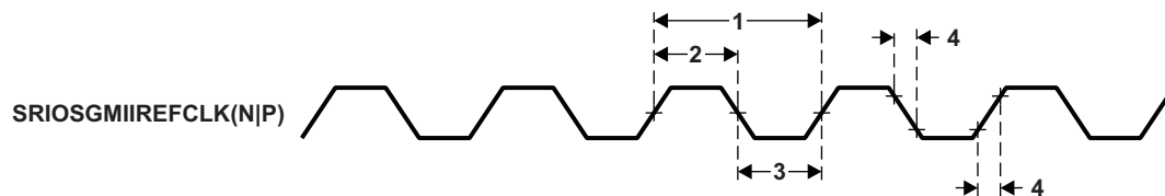
Figure 7-43. SRIOSGMIREFCLK(N|P) Timing
