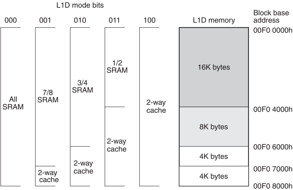
Figure 5-3 TMS320C6672 L1D Memory Configurations
