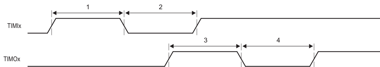
Figure 7-56 Timer Timing
