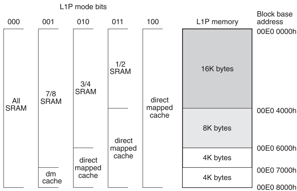
Figure 5-2 TMS320C6672 L1P Memory Configurations
