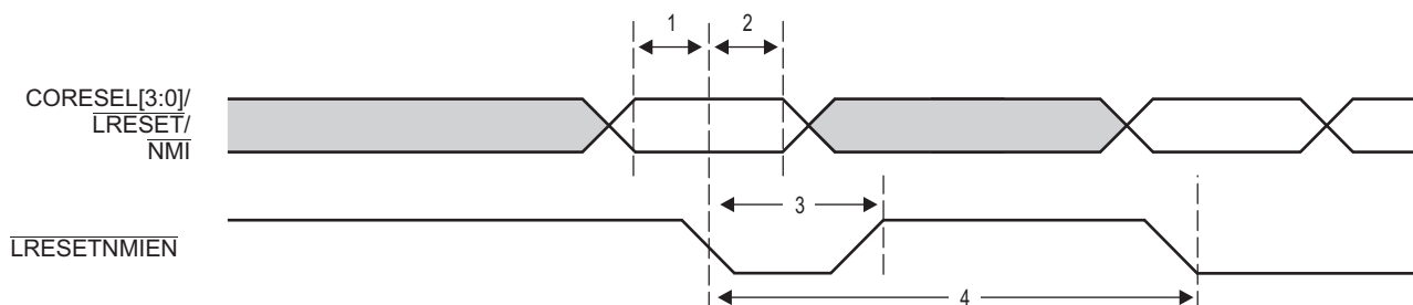
Figure 7-34 NMI and Local Reset Timing
