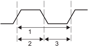
Figure 7-45 HyperLink Station Management Transmit Timing
