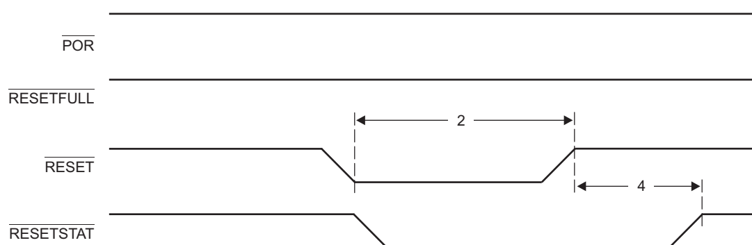
Figure 7-9 Soft/Hard-Reset Timing
