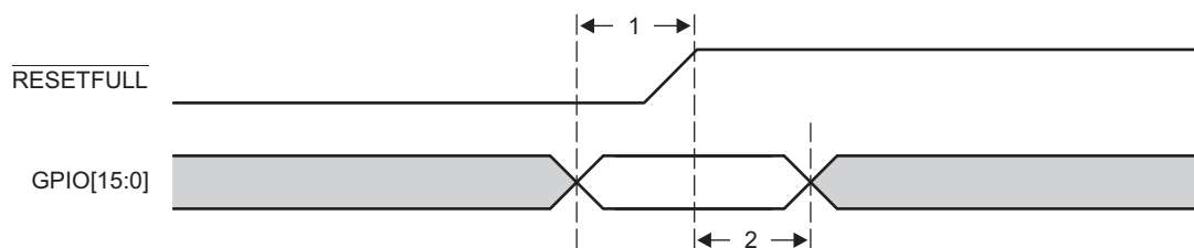
Figure 7-10 Boot Configuration Timing
