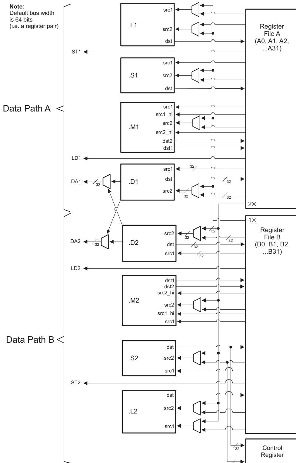
Figure 2-1 TMS320C6672 DSP Core Data Paths
