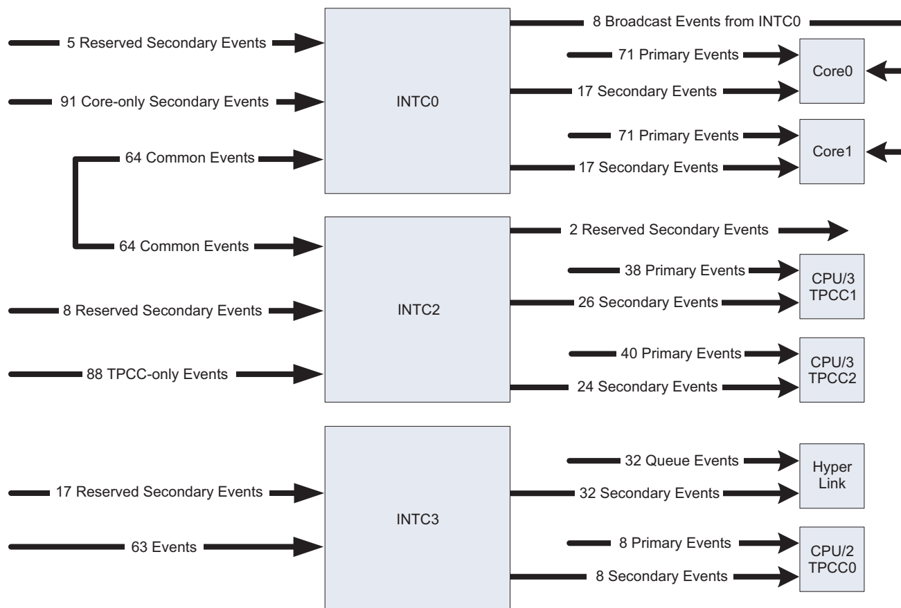
Figure 7-33 TMS320C6672 Interrupt Topology
