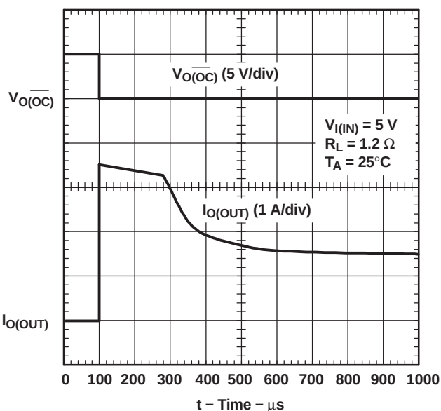
Figure 17. 1.2-Ω Load Connected to an Enabled TPS2022 Device
