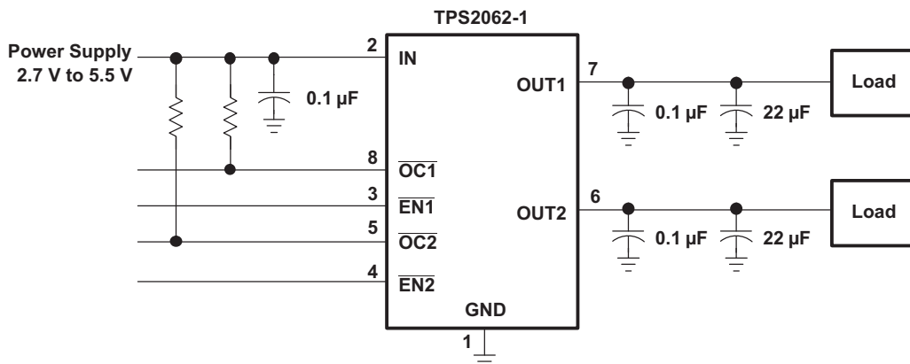
Figure 23. Typical Application
