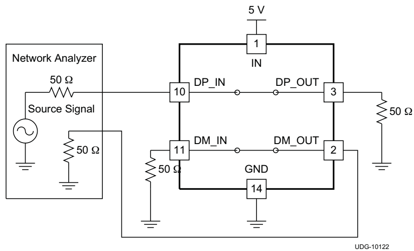
Figure 36. ON State Cross Channel Isolation ( X_{TALK} )
