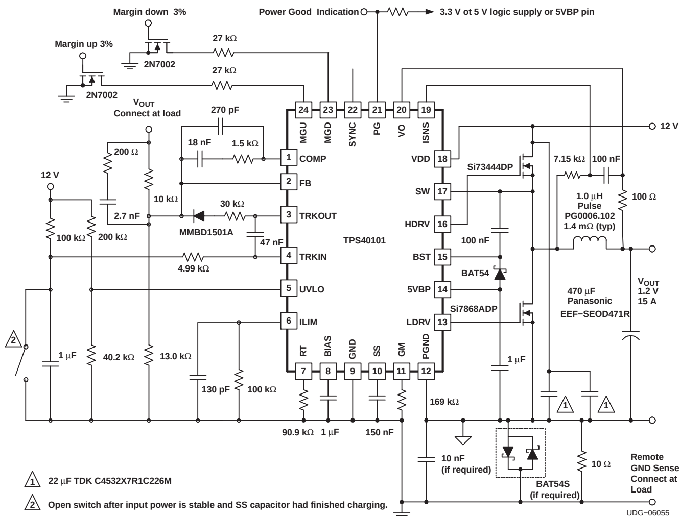
Figure 38. 500-kHz, 12-V to 1.2-V Converter With Tracking Startup Capability and Remote Sensing
