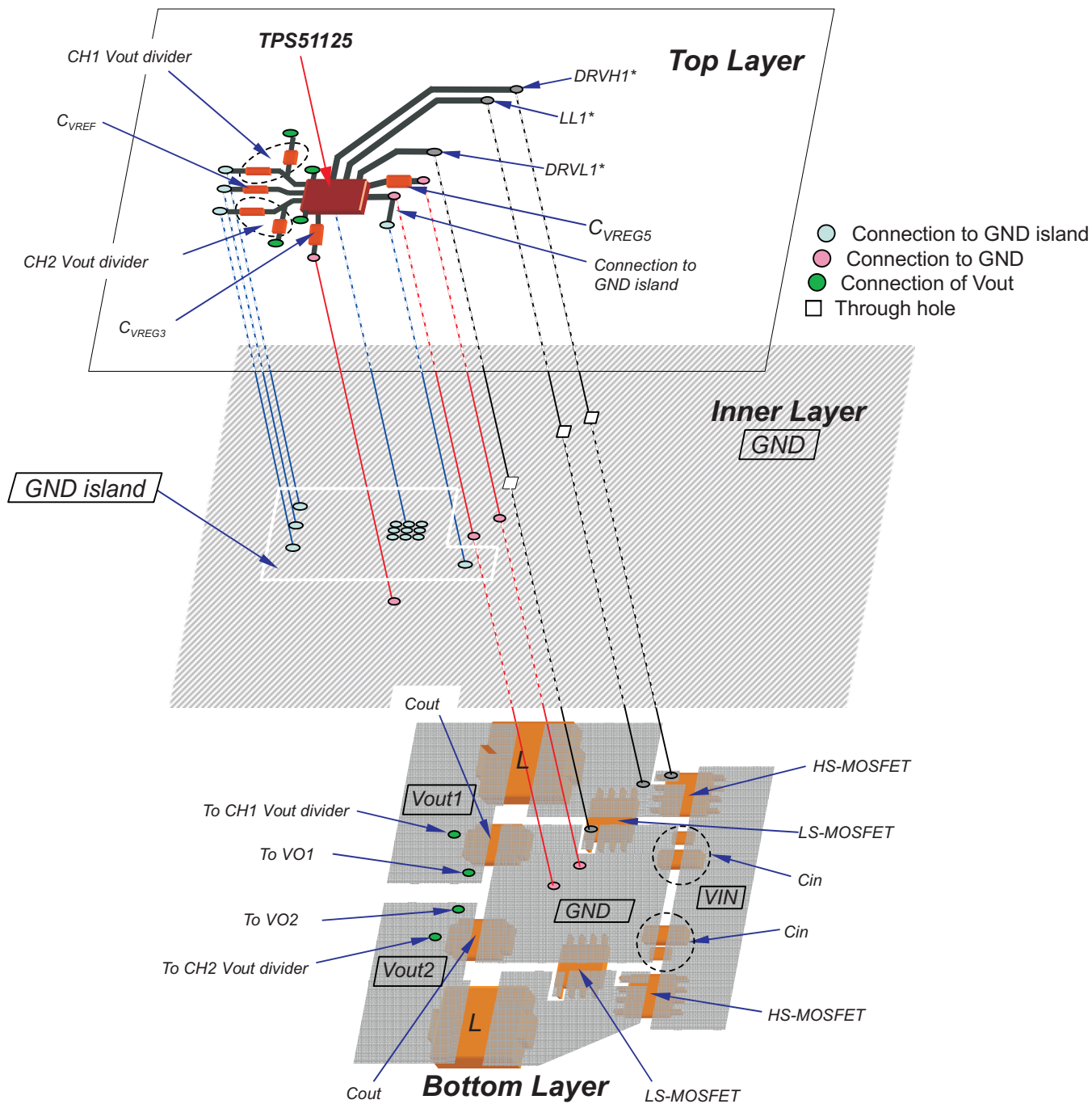
Figure 41. PCB Layout
