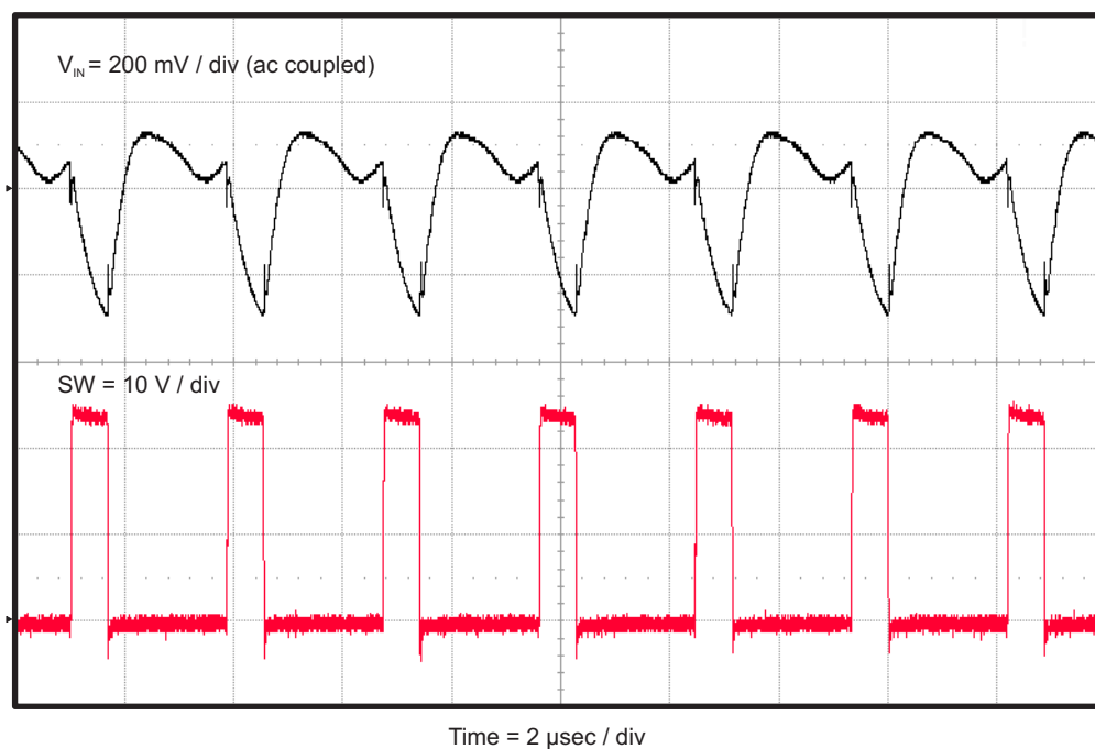
Figure 10. TPS54335AEVM-010 Input Ripple
