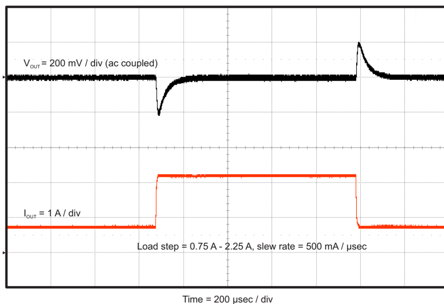
Figure 5. TPS54335AEVM-010 Transient Response
