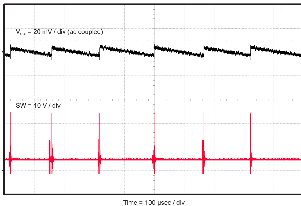
Figure 9. TPS54335AEVM-010 Output Ripple, I_{OUT} = 0 A
