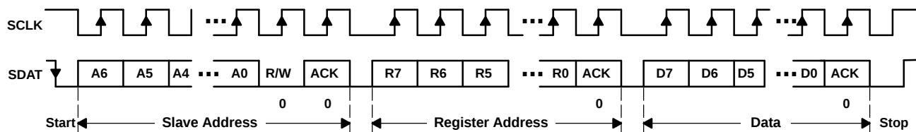
Figure 40. Serial Interface WRITE to TPS65010 Device
