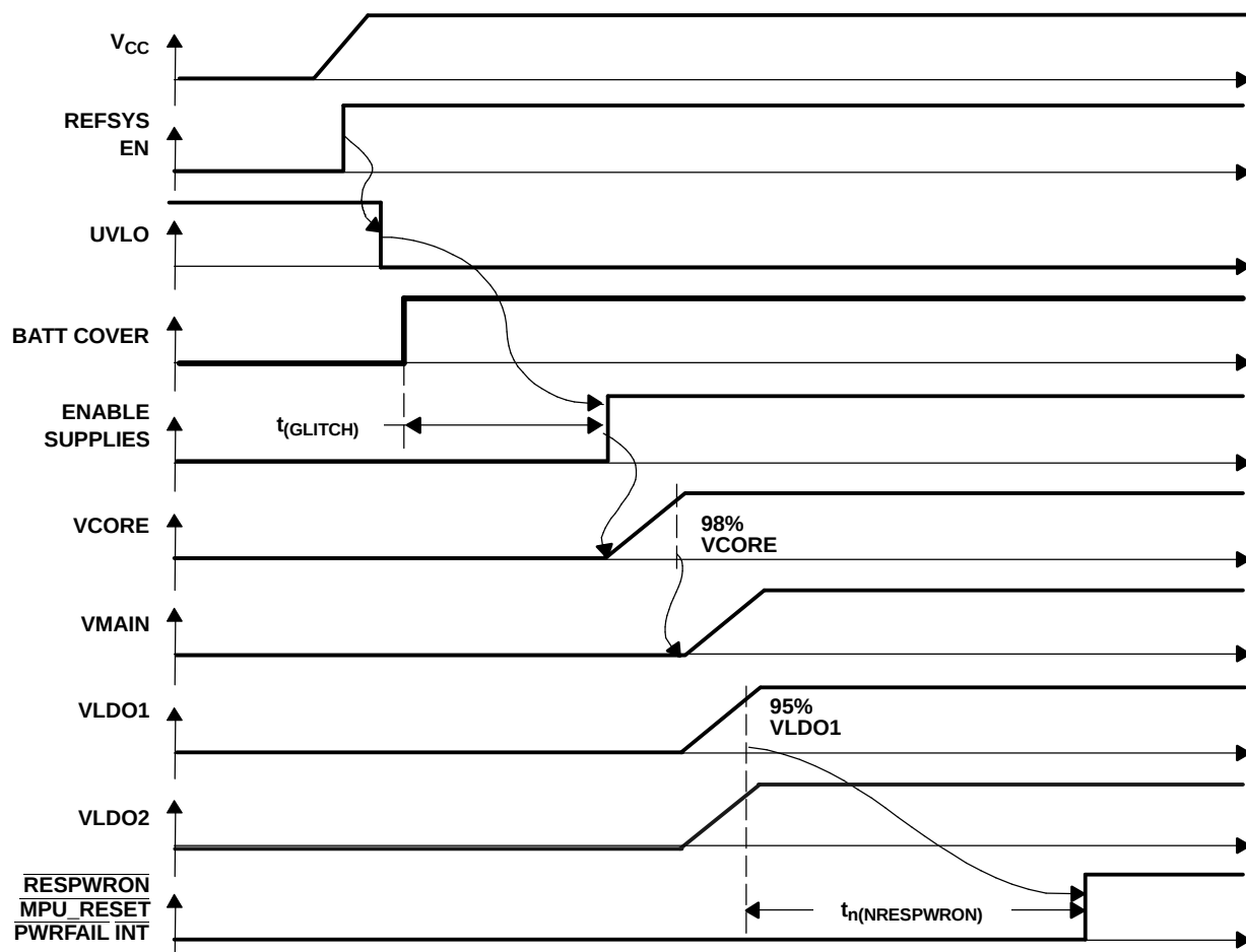
Figure 32. State 1 to State 2 Transition (PS_SEQ=0, V_{CC} > V_{UVLO} + HYST )
