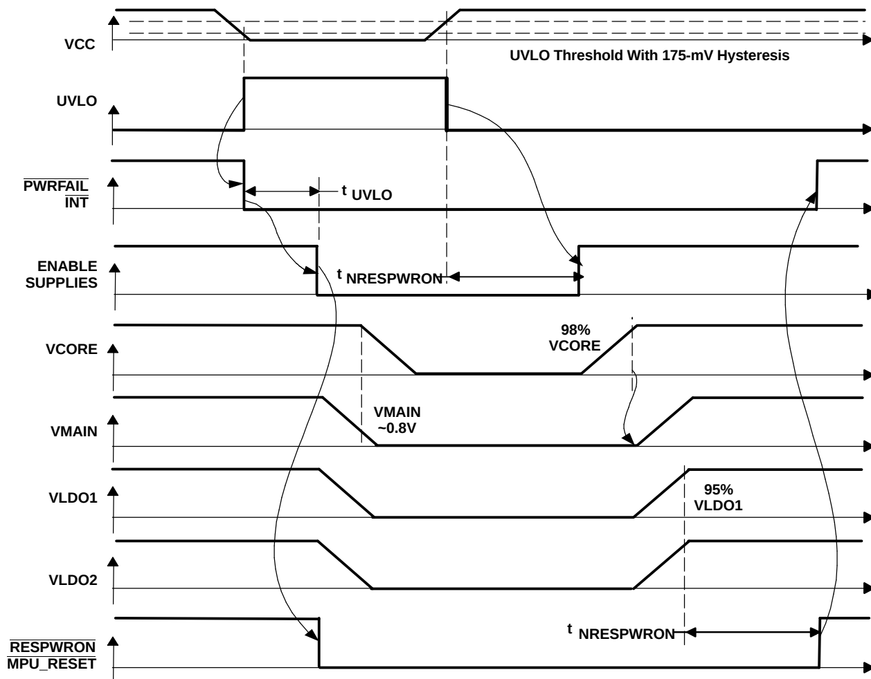
Figure 34. State2-State4-State 2 Transition
