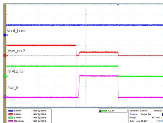
Figure 25. Power Switch No Load to 1- \Omega Transient Response
