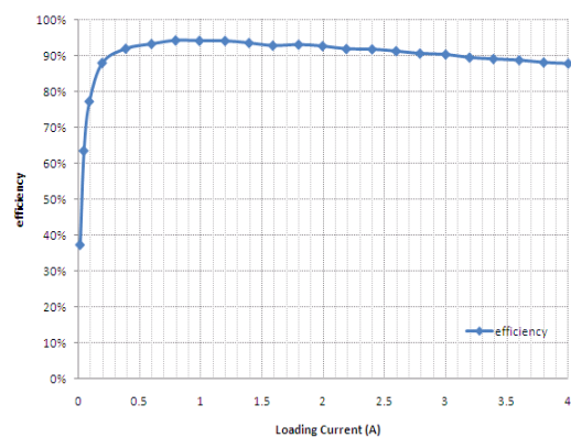
Figure 13. Buck Efficiency
