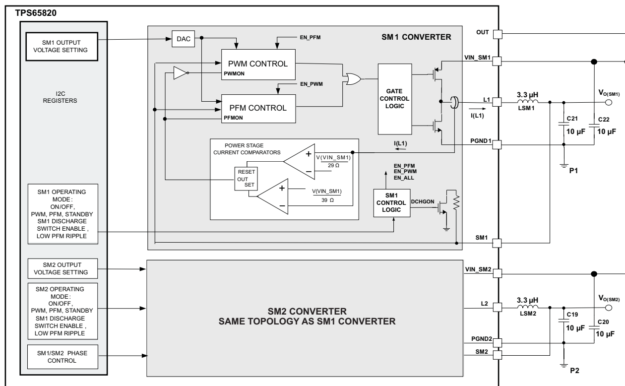
Figure 42. SM1/SM2 Converter
