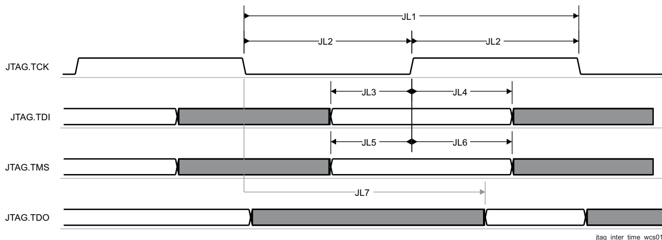
Figure 12-5. JTAG Interface Timing
