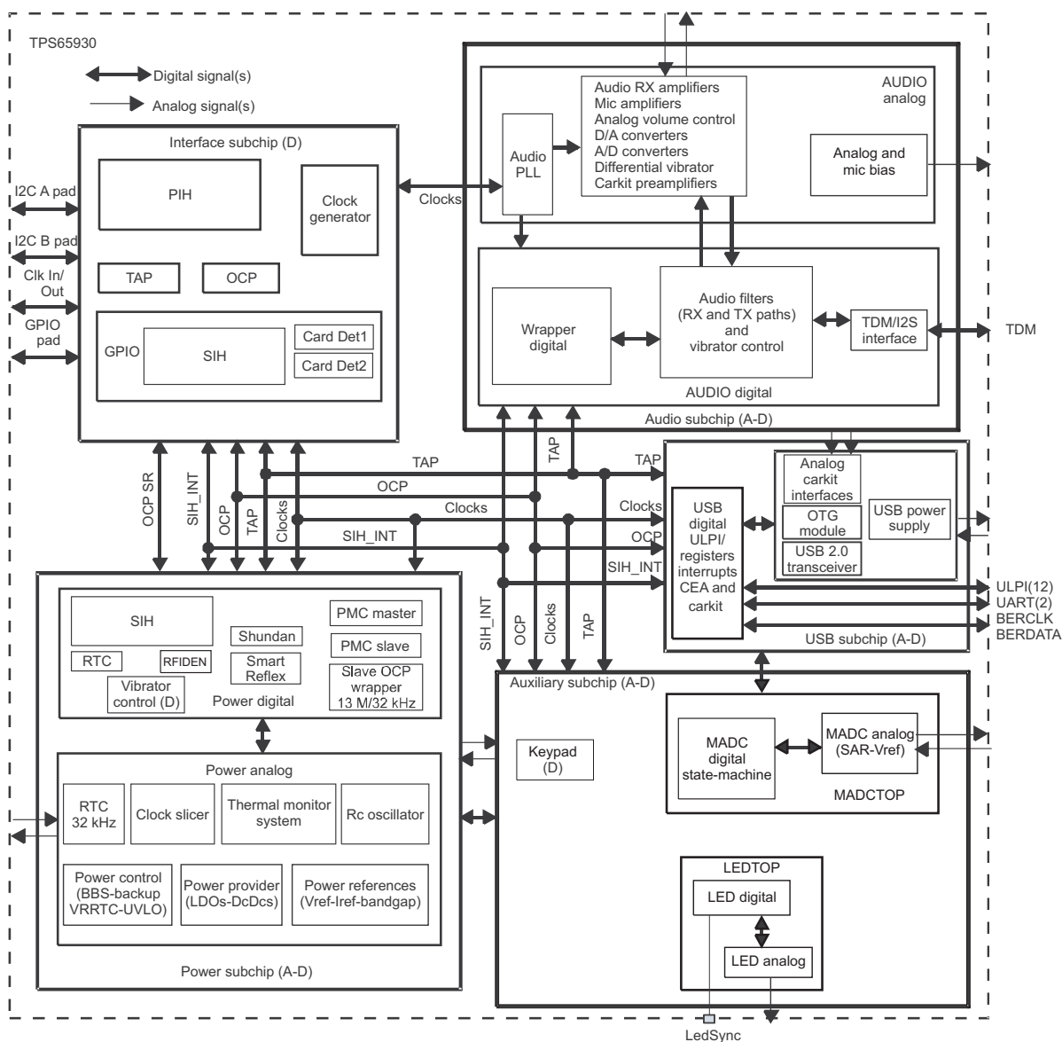
Figure 1-2. TPS65930 Block Diagram
