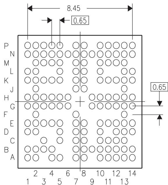
Figure 15-2. TPS65920/TPS65930 Mechanical Package Bottom View
