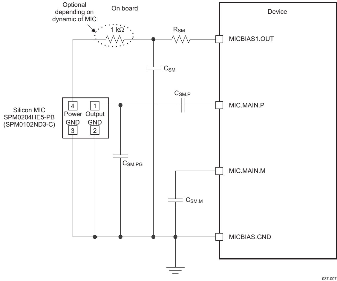
Figure 6-8. Silicon Microphone
