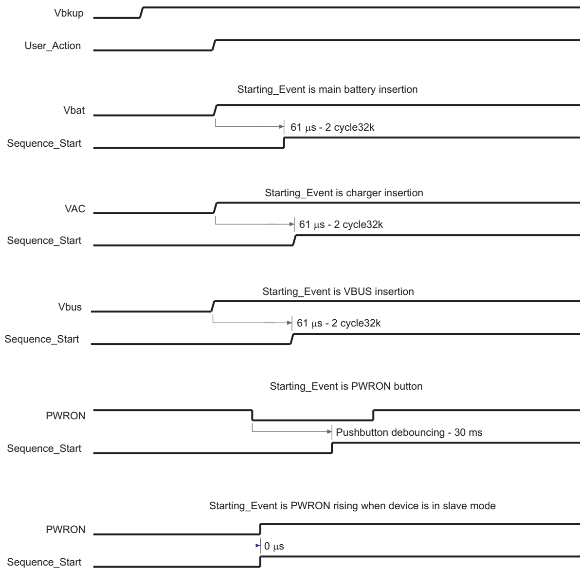
Figure 4-8. Timing Before Sequence Start
