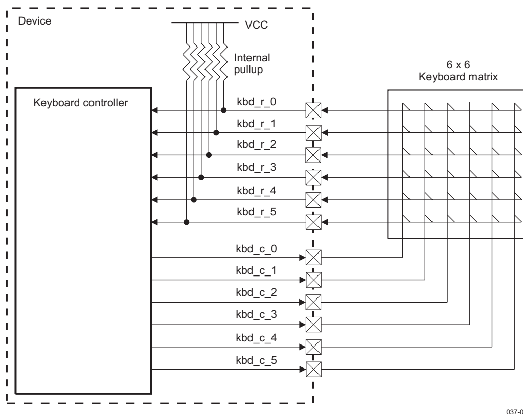
Figure 10-1. Keyboard Connection
