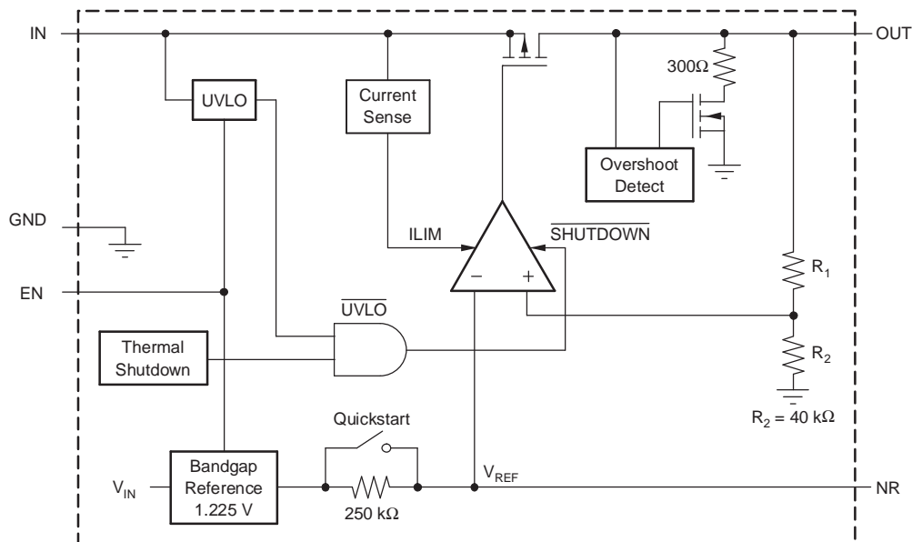
FUNCTIONAL BLOCK DIAGRAM—FIXED VERSION
