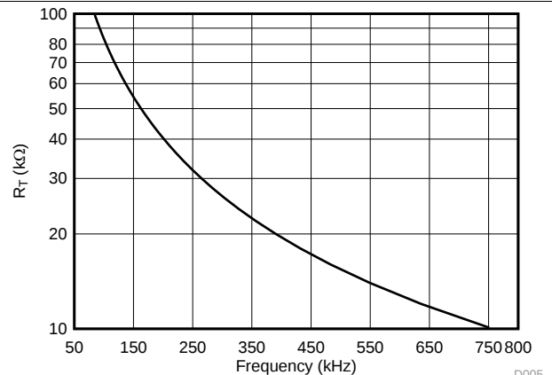
Figure 6. Timing Resistance ( R_T ) vs Switching Frequency
