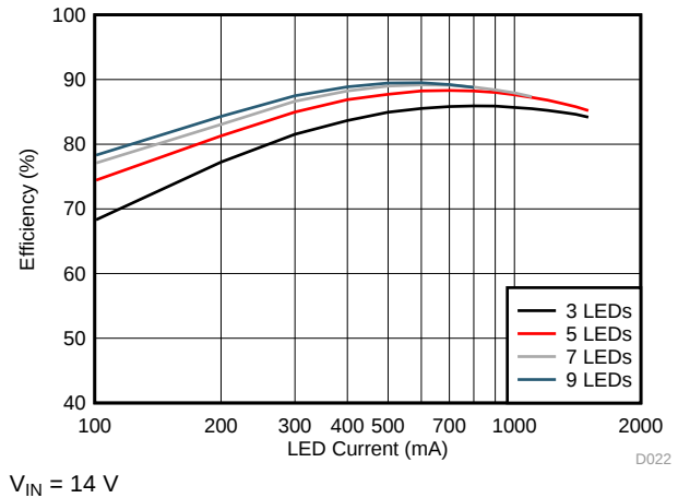
Figure 56. Efficiency
