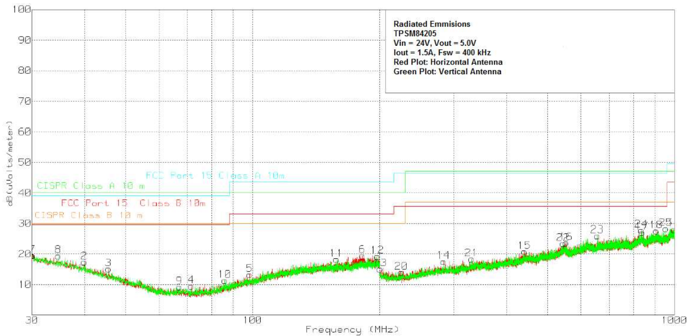
Figure 26. Radiated Emissions 12-V Input, 5.0-V Output, 1.5-A Load, Horizontal and Vertical Antenna
