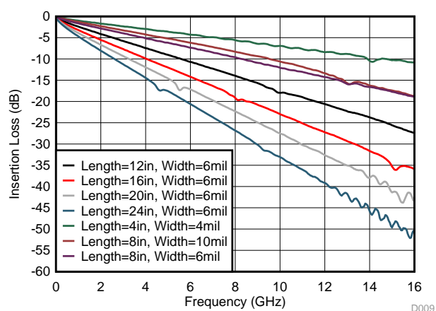
Figure 29. Insertion Loss of FR4 PCB Traces
