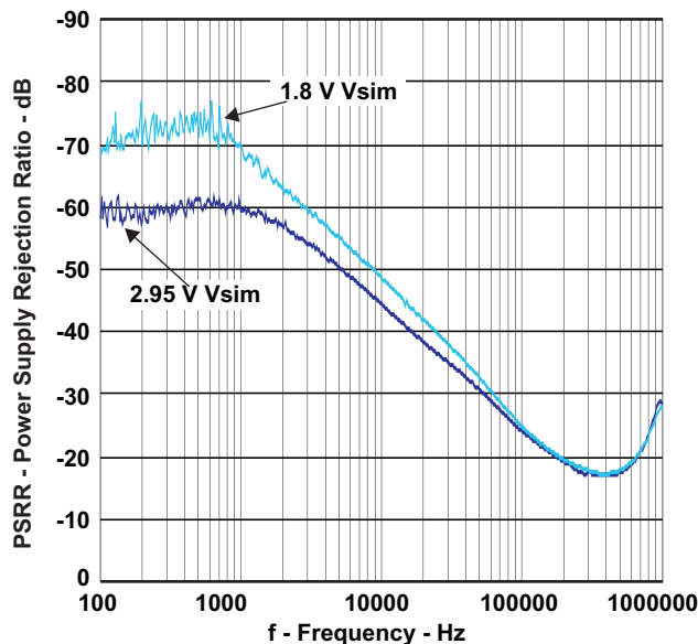
Figure 10. PSRR
