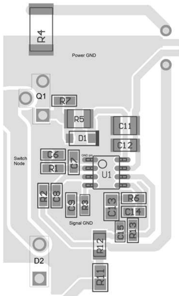
Figure 41. Recommended Layout for UCC28180
