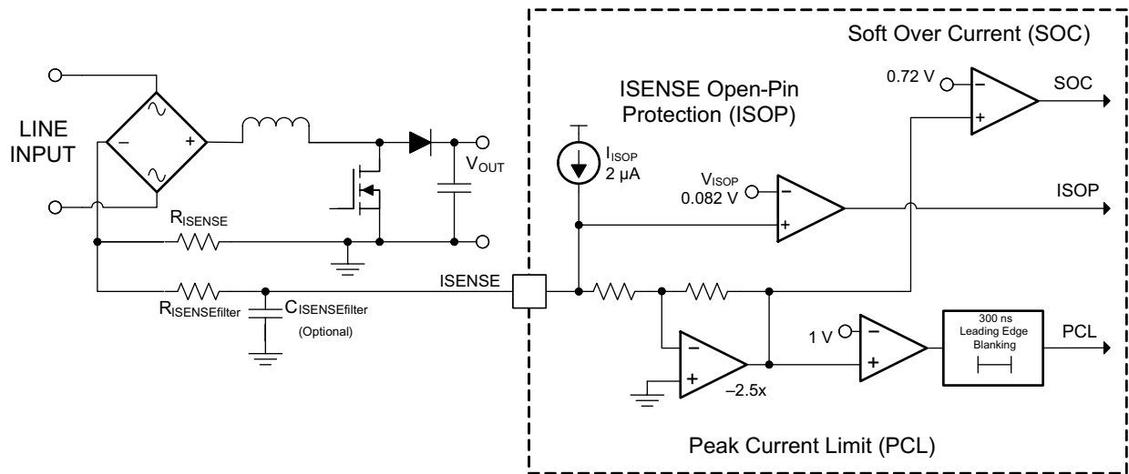
Figure 26. Soft Overcurrent/Peak-Current Limit
