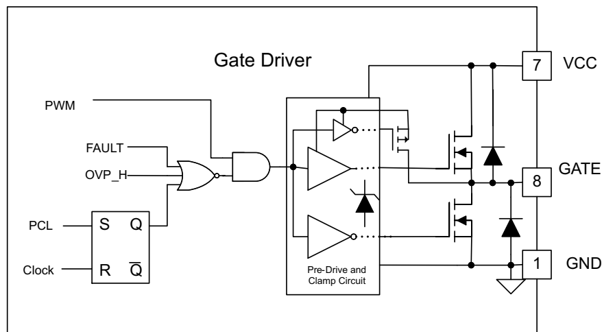
Figure 27. Gate Driver
