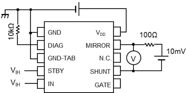
Figure 11.4 Test Circuit 4
