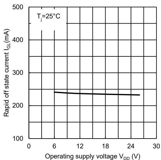
I_{GL} - V_{DD}
