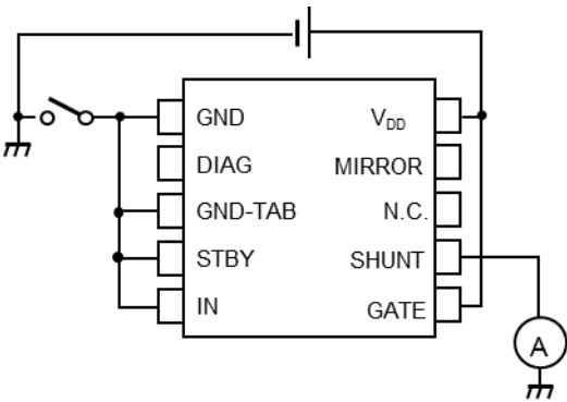
Figure 11.3 Test Circuit 3
