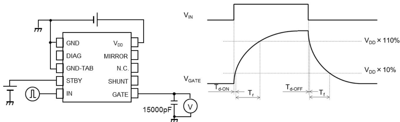
Figure 11.2 Test circuit 2
