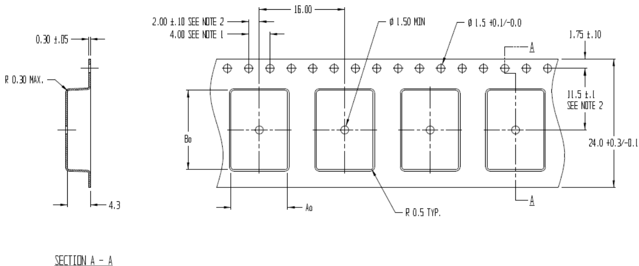
Figure 12: NINA-W101 tape dimension
