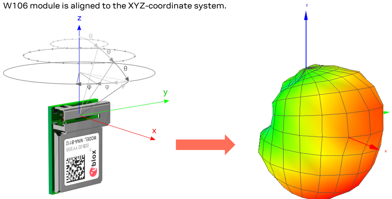
Figure 4: Measurement procedure for determining radiation patterns. A measurement is taken at every dot in the figure to the left, and is represented as a grid point in the radiation pattern to the right.
