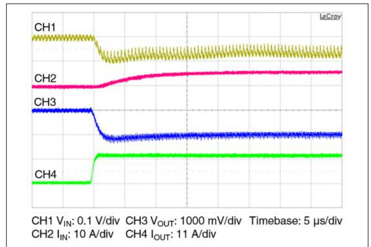
Figure 11 — 0 A–12.0 A transient response: C_{IN} = 330 \mu F , I_{IN} measured prior to C_{IN} , no external C_{OUT}
