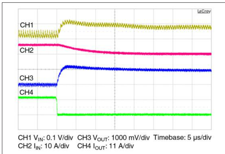
Figure 12 — 12.0 A–0 A transient response: C_{IN} = 330 \mu F , I_{IN} measured prior to C_{IN} , no external C_{OUT}
