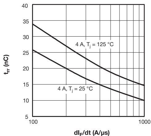
Fig. 7 - Typical Reverse Recovery Time vs. di/dt
