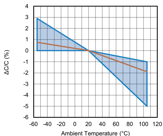
Capacitance as a function of ambient temperature (typical curve)
