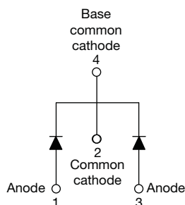
3L TO-220AB
