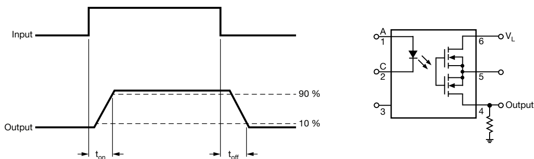
Fig. 2 - Timing Schematic
