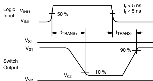
Figure 4. Transition Time
