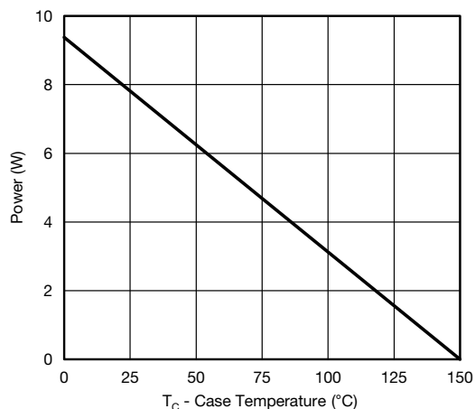
Power, Junction-to-Foot
