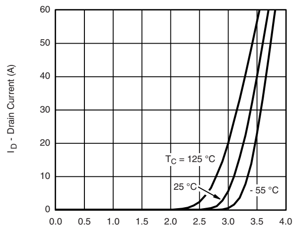
T_C = 125^\circ\text{C} 25^\circ\text{C} -55^\circ\text{C} I_D - Drain Current (A) V_{GS} - Gate-to-Source Voltage (V) Transfer Characteristics
