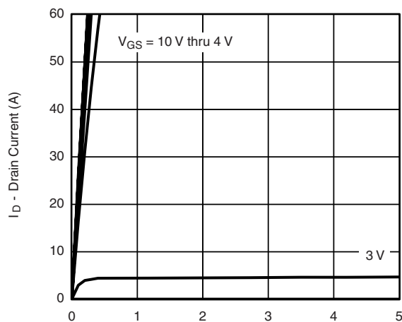
V_{GS} = 10\ \text{V} thru 4\ \text{V} I_D - Drain Current (A) V_{DS} - Drain-to-Source Voltage (V) Output Characteristics
