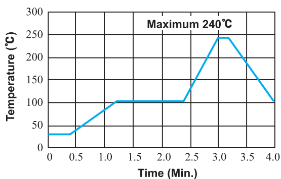
Soldering Profile for Non-RoHS Type
