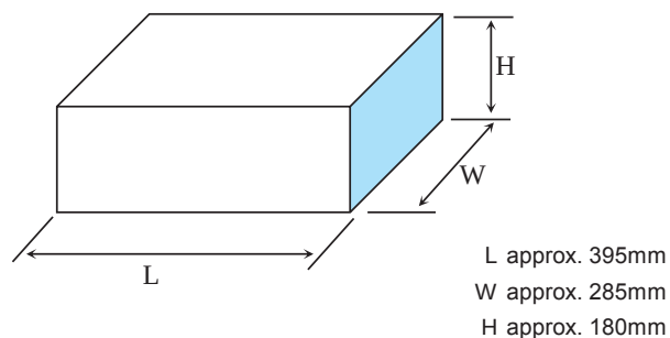
Carton size of bulk packing
