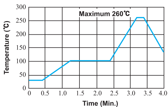
Soldering Profile for RoHS Type
