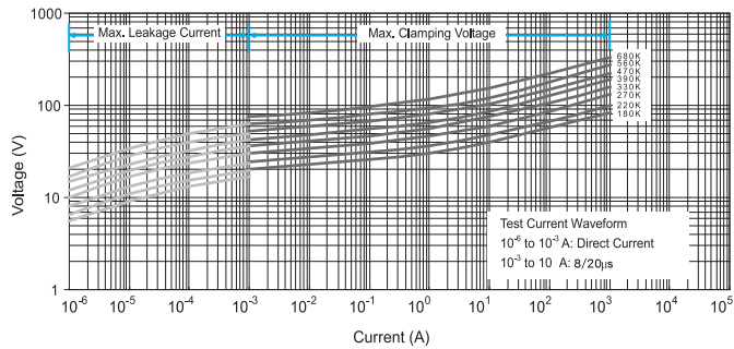
V-I Curve for SR180K~680K10D(E) Series
