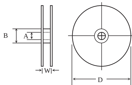
Reel Dimension
