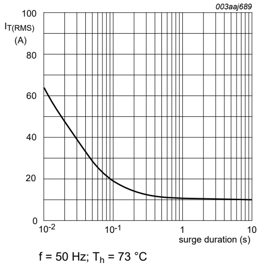
Fig. 2. RMS on-state current as a function of surge duration; maximum values f = 50\text{ Hz} ; T_{\text{h}} = 73\text{ }^{\circ}\text{C}
