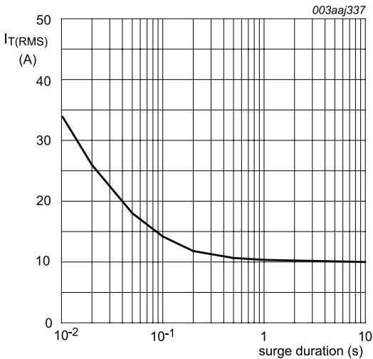
f = 50\text{Hz} ; T_{mb} = 131\text{ }^{\circ}\text{C} Fig. 2. RMS on-state current as a function of surge duration; maximum values
