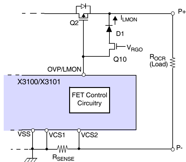
Figure 5. Over-Current Protection
