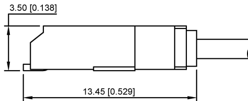
Assembly Layout
