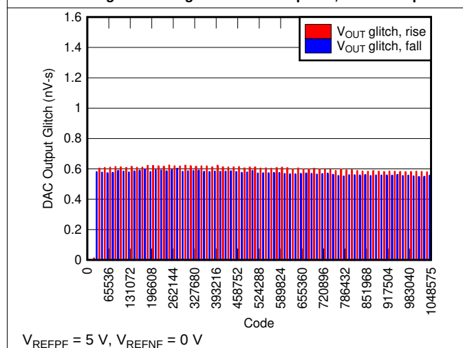
Figure 35. Segment Glitch Impulse, 1-LSB Step
