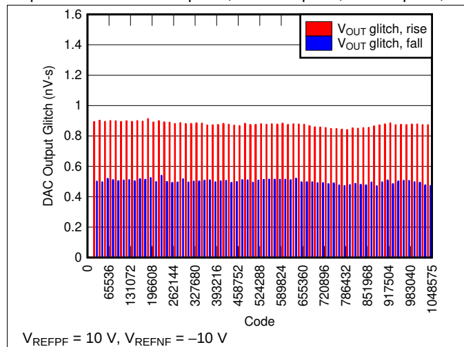
Figure 33. Segment Glitch Impulse, 1-LSB Step
