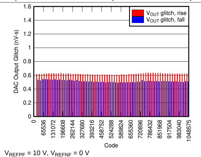
Figure 34. Segment Glitch Impulse, 1-LSB Step
