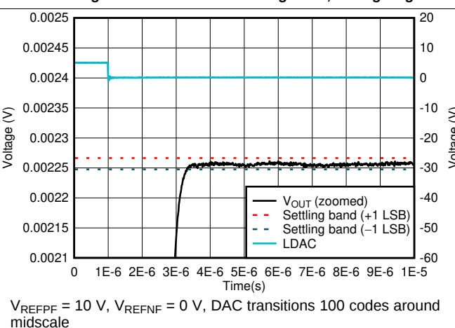
Figure 38. 100 Codes Settling Time, Rising Edge
