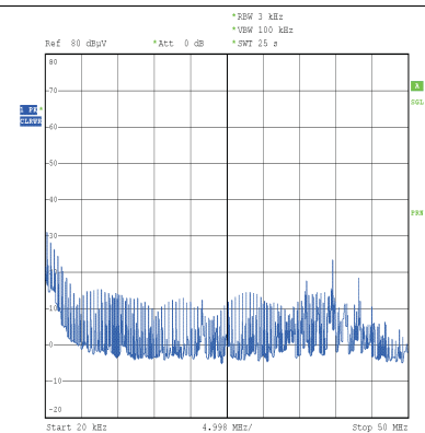
Figure 6. Emissions Spectrum to 50 MHz
