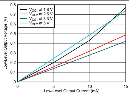
Figure 7-14. Low-Level Output Voltage vs Low-Level Output Current
