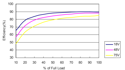
MJWI20-48S033 Efficiency vs Load Current
