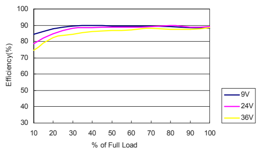
MJWI20-24S12 Efficiency vs Load Current
