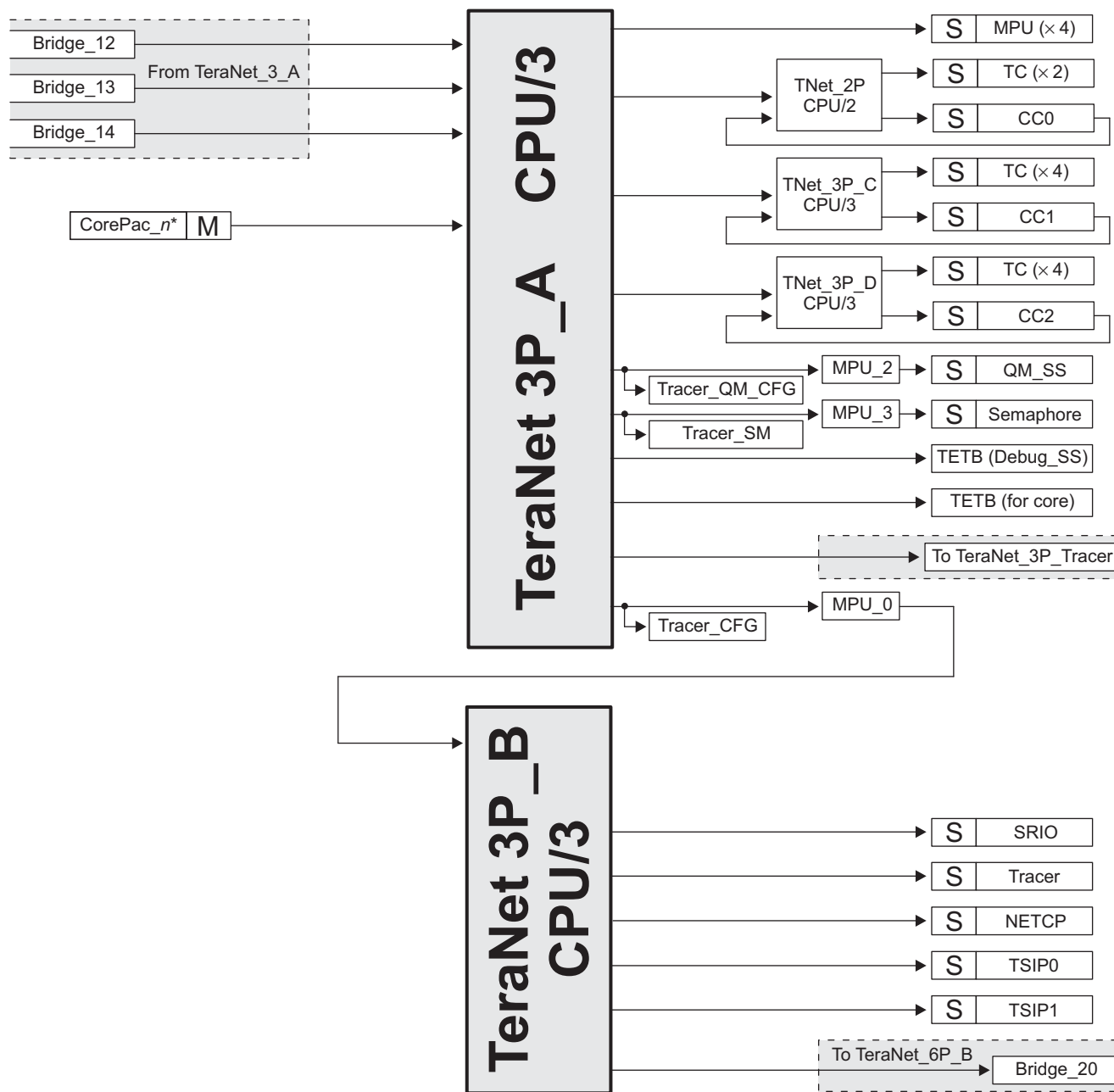
Figure 4-3 TeraNet 3P_A & B for C6674
