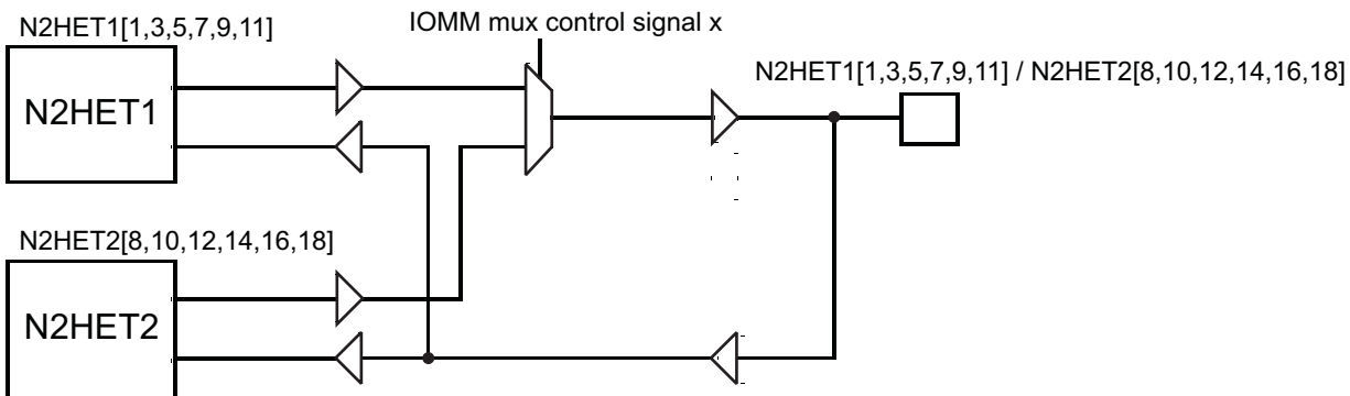
Figure 7-18. N2HET Monitoring
